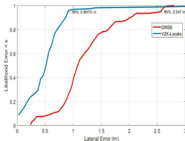
Figure 4 COMPARISON OF V2X-LOCATE WITH GNSS IN IDEAL OPEN SKY CONDITIONS
